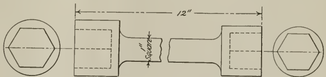
DETAILS OF DOUGLE SOCKET WRENCH.
